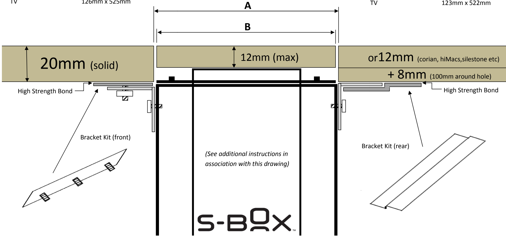
MASTER DRAWING FOR INSTALLING S-BOX™ WITH CUSTOM TOP IN 20mm WORKTOP MATERIAL
